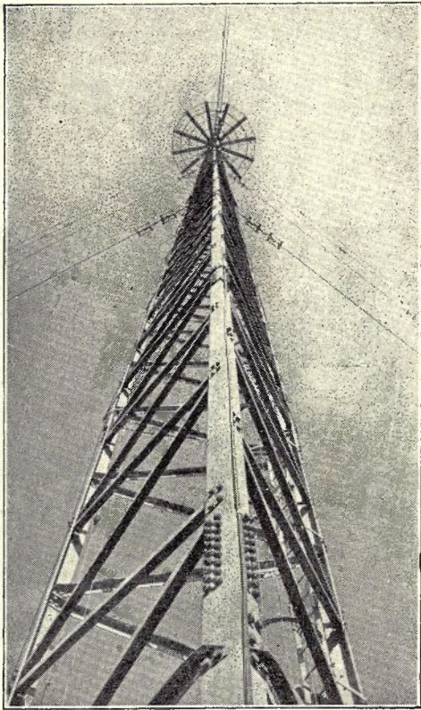
Fig. 10.—Loaded Radiator.
