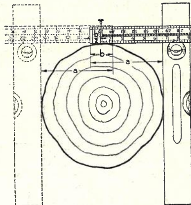
Fig. 5.—Striking Pole Centre.
