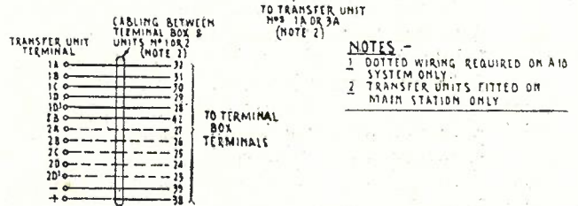
Fig. 4.—Terminal Box Connections.
