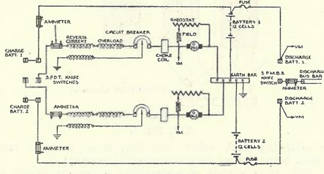
POWER CIRCUIT CARRIER REPEATER STATION Q. 8, Fig. 1.
