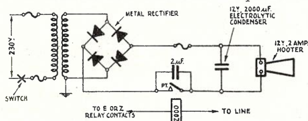
Fig. 3.—Hooter Circuits.
