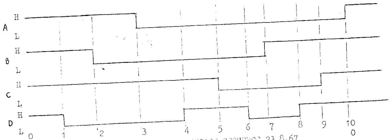
WAVEFORMS FOR DECADE SEQUENCE 23.8.67
